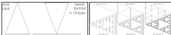
Figure 5: Lindenmayer system axiom Gasket
