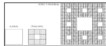
Figure 7: Sierpinski carpet
