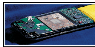
Figure 2: Fractal Antenna
